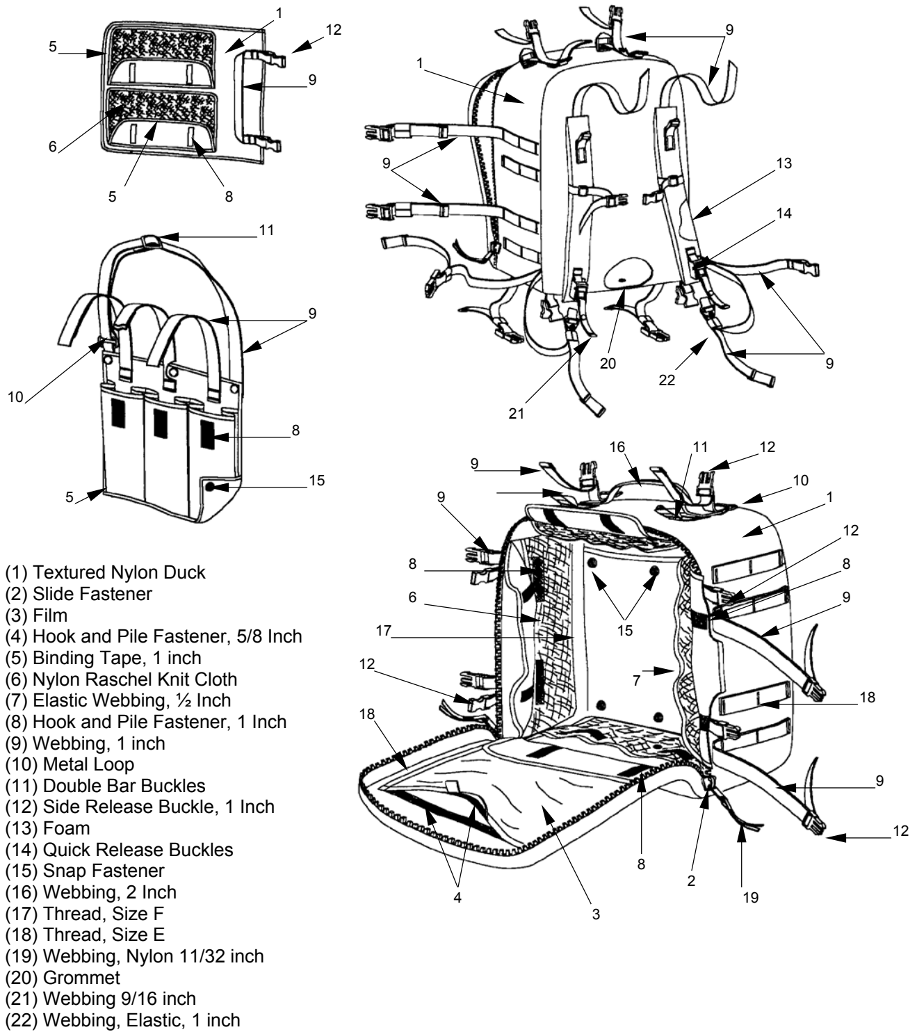
Figure 27-11 (Page 1). Medic Bag
