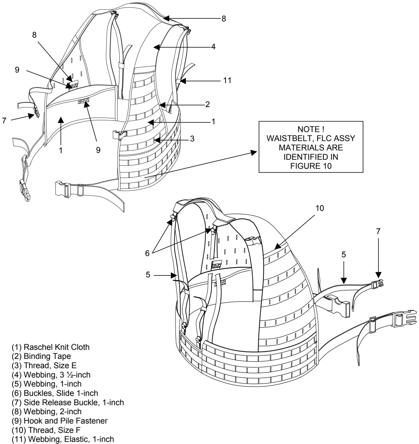
Figure 27-2. Vest, Fighting Load Carrier
