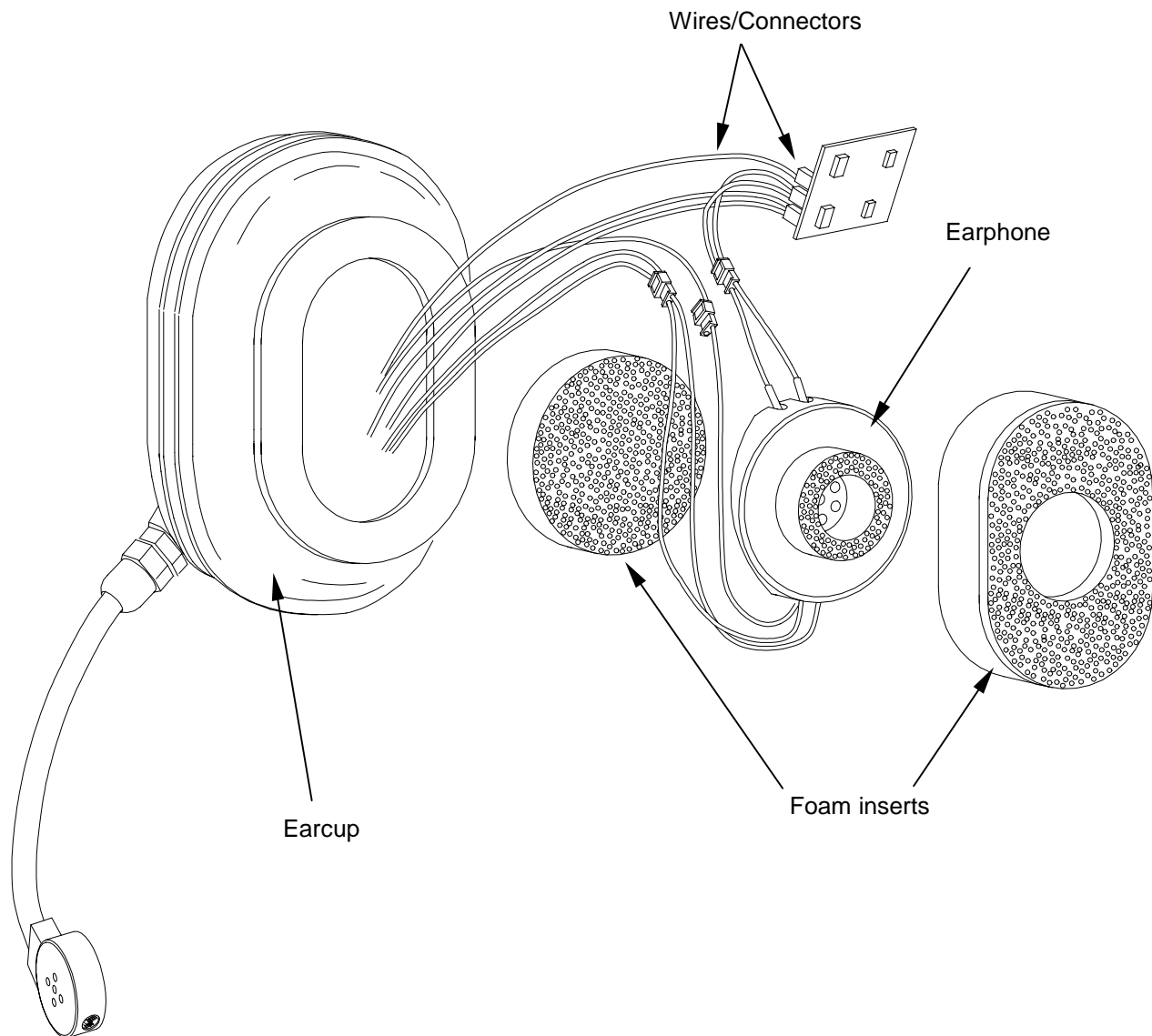
Figure 26-12. Headset Assembly
