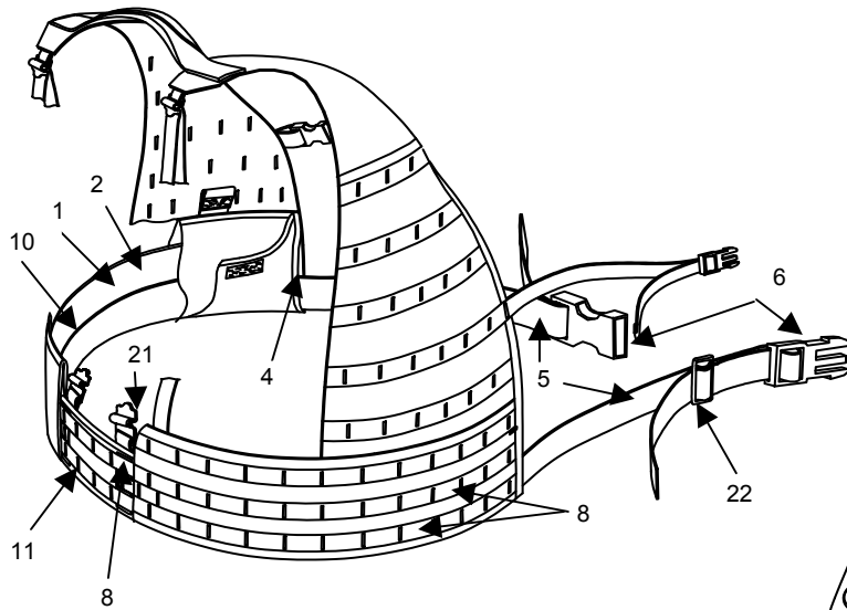
WAISTBELT, FLC ASSY
